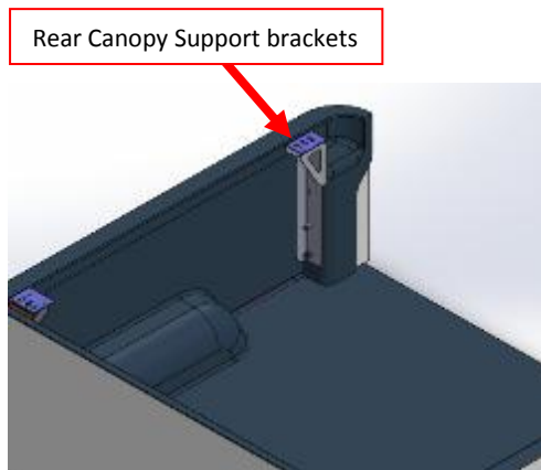
Figure 7: Rear Canopy Support Bracket Position
