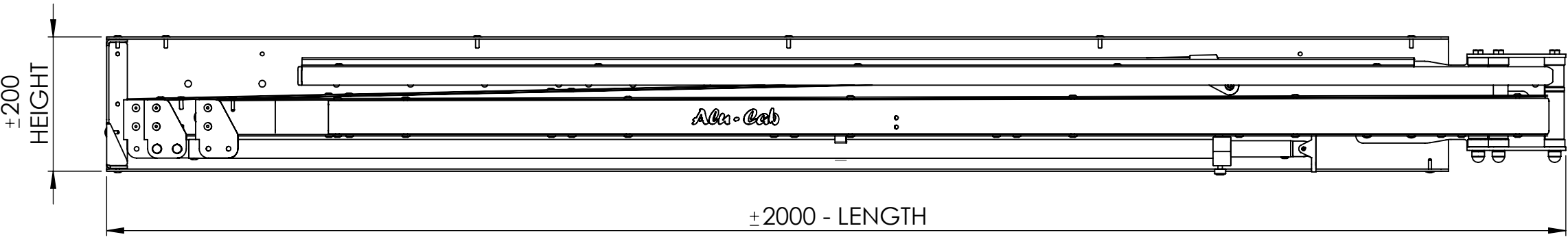
FRONT VIEW
